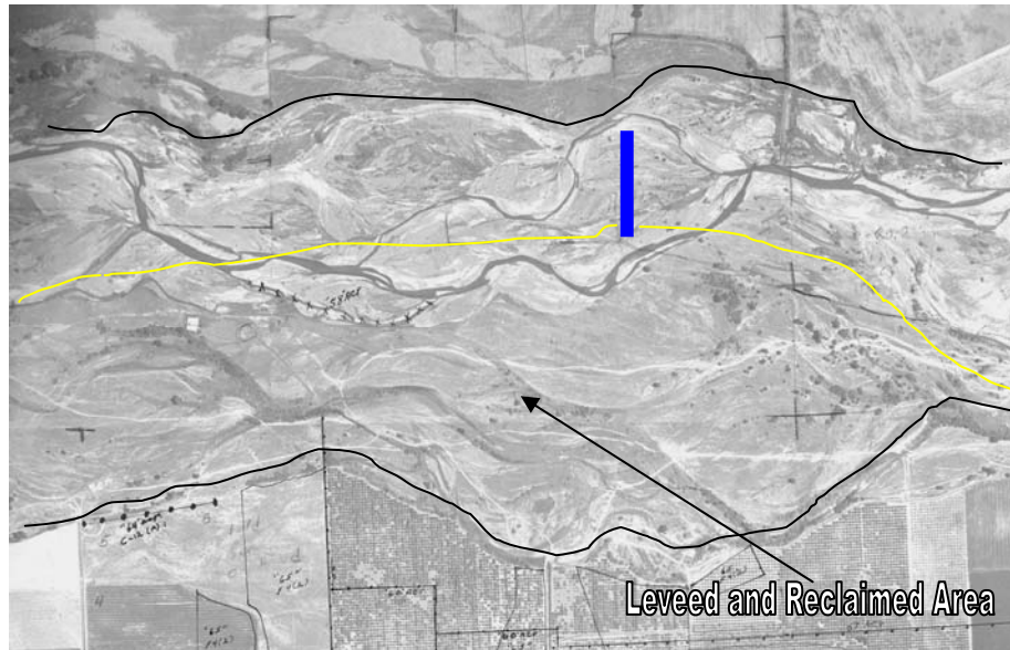
Image Comparison 4c. Thomes Creek at the Interstate 5 crossing site in 1952 (above) and 1994 (bottom). Note the braided stream condition in both images. The Interstate 5 Bridge locations and lengths are shown as a blue bar. The extent of overflow patterns in 1952 are shown by the black lines and the 1994 extent of stream constriction is shown by the yellow line. Comparing these images show the extent of channel constriction. (The feature to the west of Interstate 5 is the Corning Canal crossing.)
